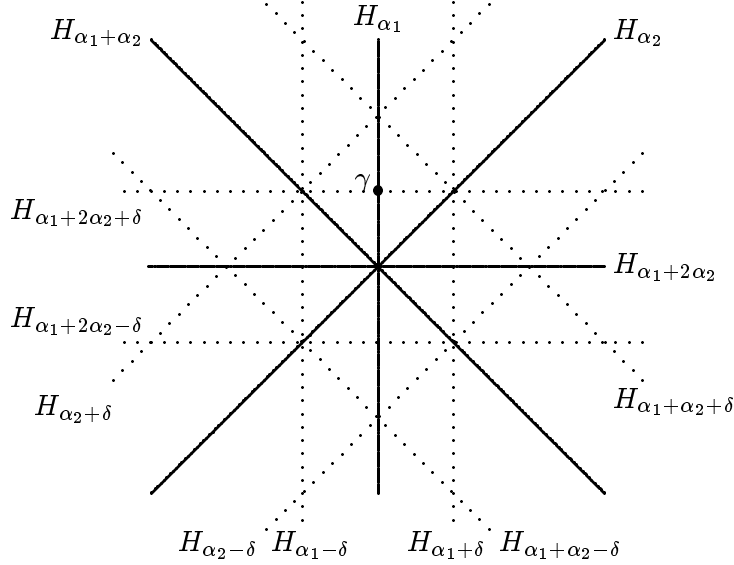
FIGURE 3. Hyperplanes and a nonintegral weight for C_2
