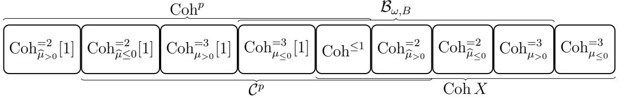
FIGURE 2. Relating the various t-structures
