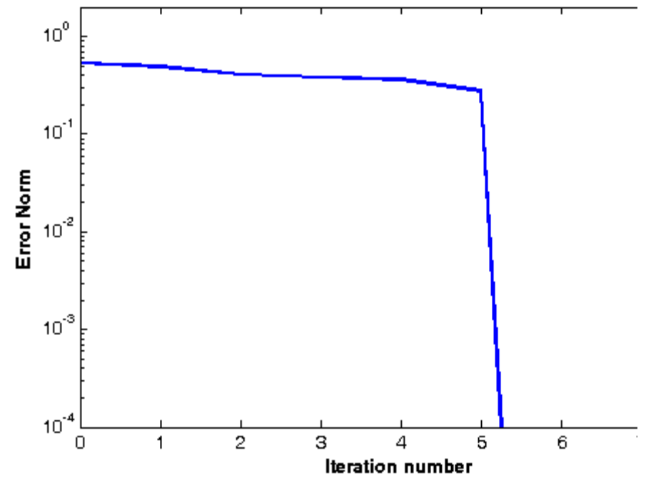
1st order upwind Convergence History
