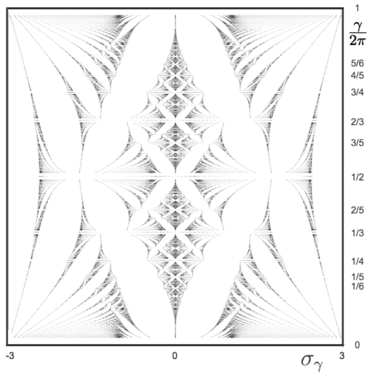
Figure 3: Hexagonal lattice.
